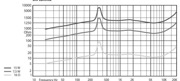
IMPEDANCE
